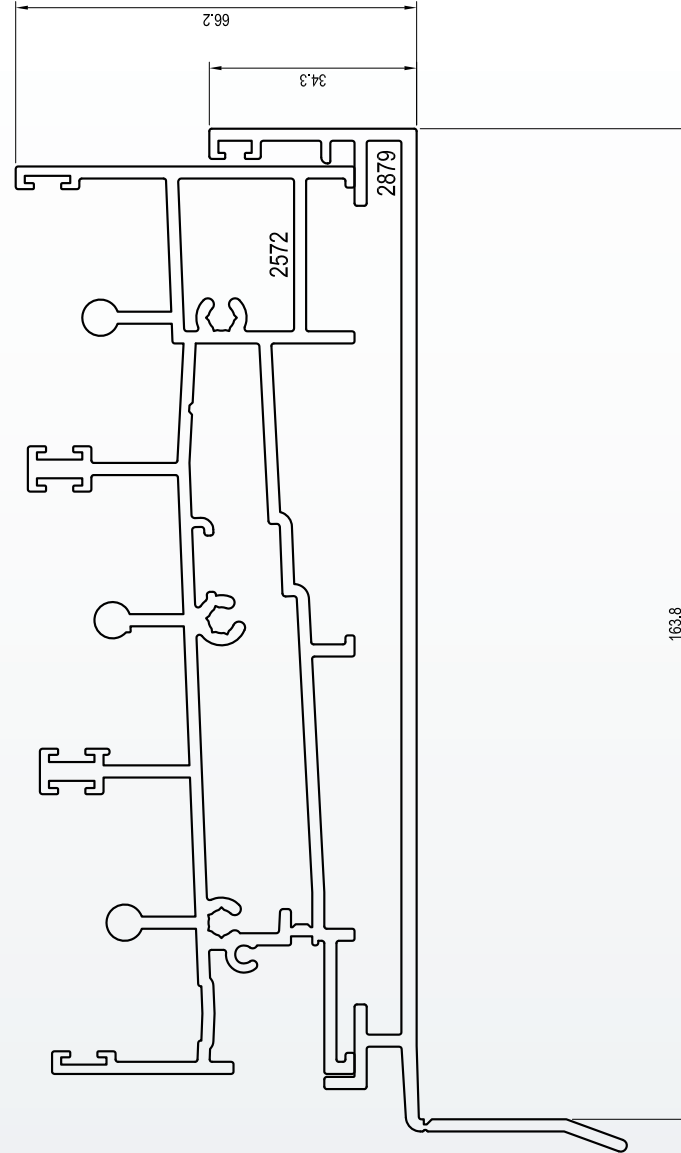
2572 SILL 3 TRACK STD WITH 2879 SUBSILL '1' 150
